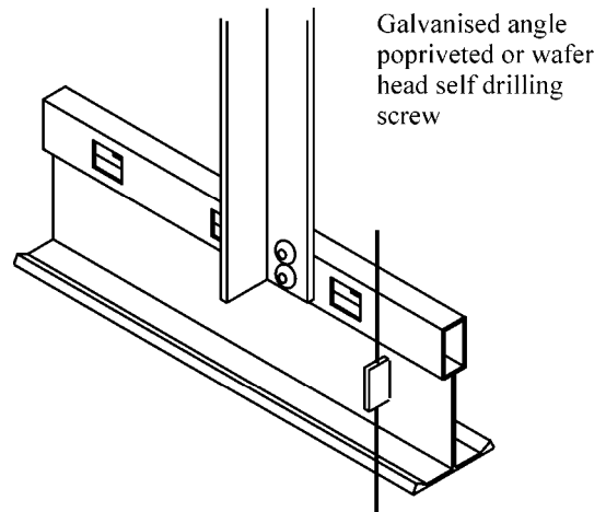
Angle Suspension
