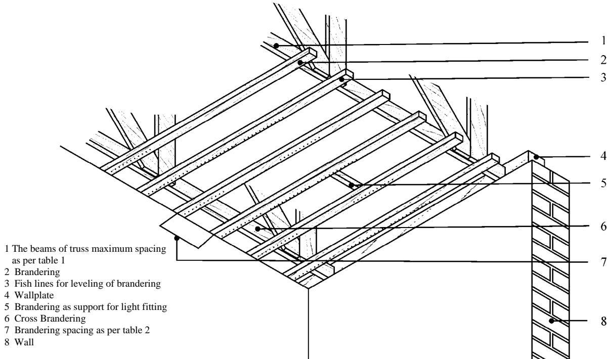
Figure 7: Installation of supporting brandering
