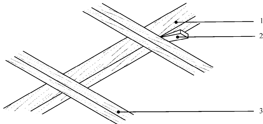
Figure 8: Levelling the brandering by wedging
